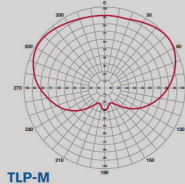
TLP-M Azimuth Gain=1.9
