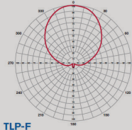
TLP-F Azimuth Gain=3.6
