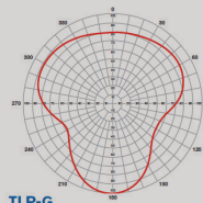
TLP-G Azimuth Gain=1.6
