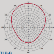
TLP-B Azimuth Gain=1.7
