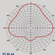
TLP-H Azimuth Gain=1.7
