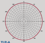
TLP-A Azimuth Gain=1.0
