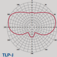
TLP-J Azimuth Gain=2.0
