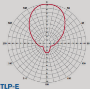
TLP-E Azimuth Gain=3.9
