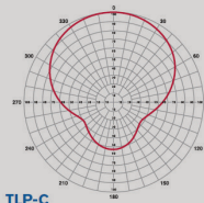
TLP-C Azimuth Gain=2.1
