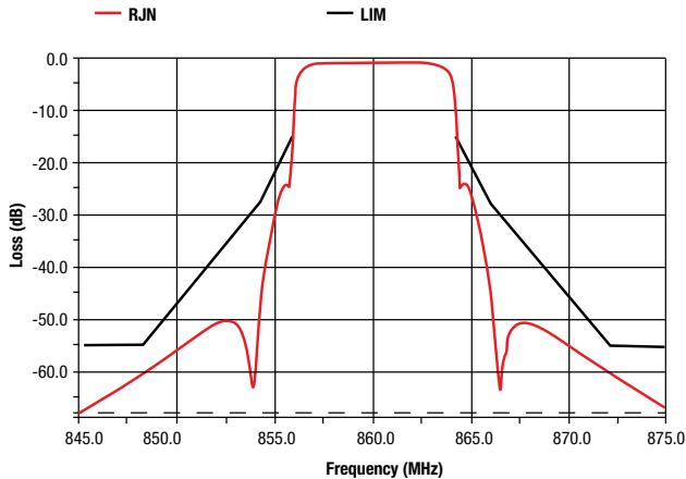
8 MHz DVB-T CRITICAL MASK
