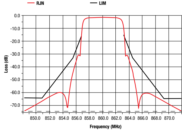
ISDB-T CRITICAL MASK
