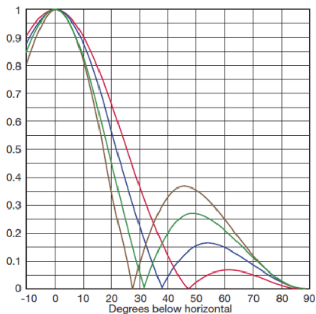
ELIVATION PATTERN: 500, 600, 700, 800 MHz
