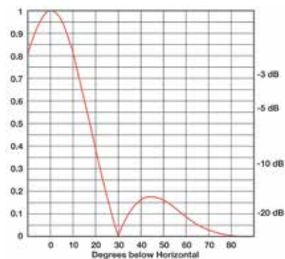
4 BAY \lambda/2
