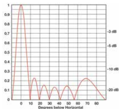
6 BAY \lambda
