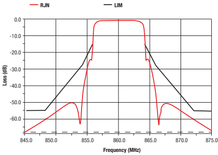
8 MHz DVB-T Critical Mask
