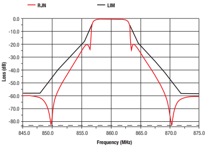
6 MHz DVB-T Non-Critical Mask
