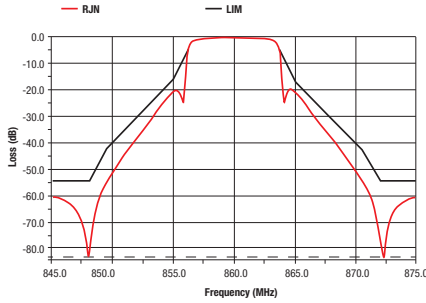
7 MHz DVB-T Non-Critical Mask
