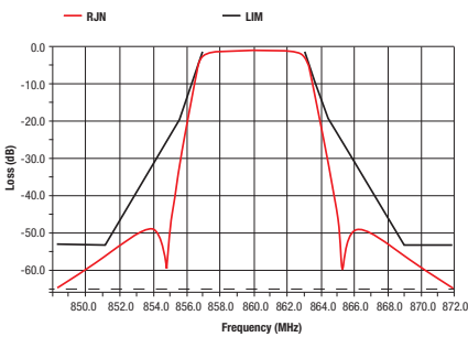
ISDB-T Non-Critical Mask
