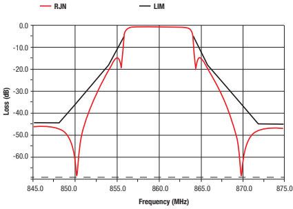
8 MHz DVB-T Non-Critical Mask
