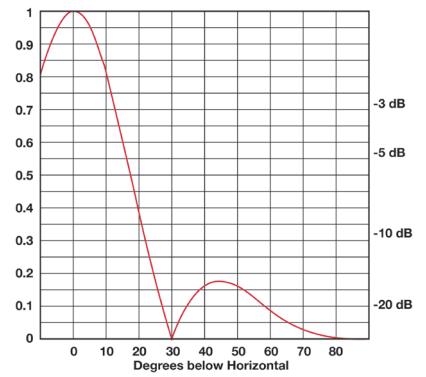
4 BAY \lambda/2
