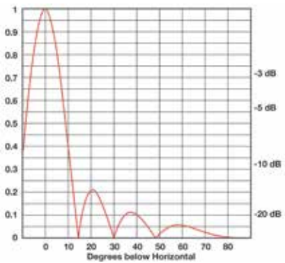
8 BAY \lambda/2
