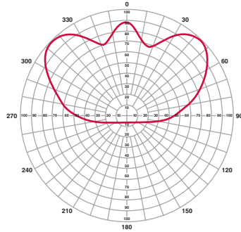
TUA-M-C2 Azimuth gain=2.9
