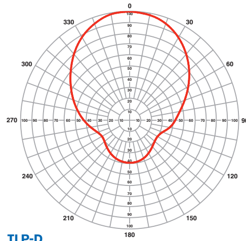
TLP-D Azimuth gain=2.9
