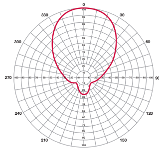
TLP-E Azimuth Gain=3.9
