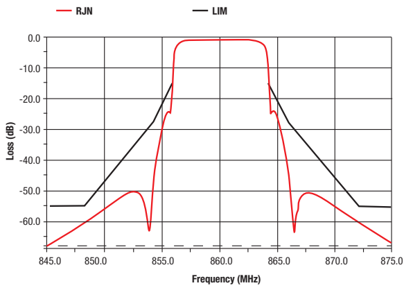
8 MHz DVB-T Critical Mask
