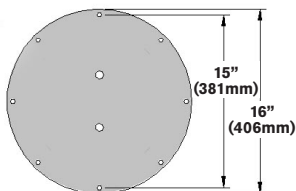
BASE FLANGE
