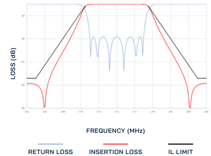
8-POLE ATSC SHARP-TUNED MASK
