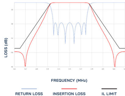
6-POLE ATSC FULL MASK
