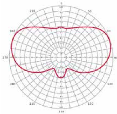
DSB-J DIRECTIVITY = 2.0
