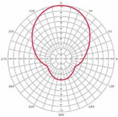
DSB-D DIRECTIVITY = 2.9
