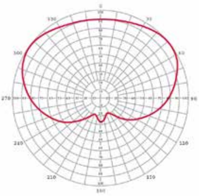
DSB-M DIRECTIVITY = 1.9
