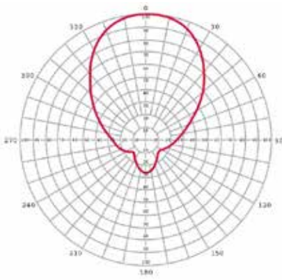
DSB-E DIRECTIVITY = 3.9
