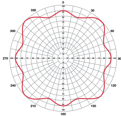
THA-04 DIRECTIVITY = 1.3
