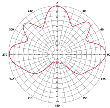
C3 DIRECTIVITY = 2.0
