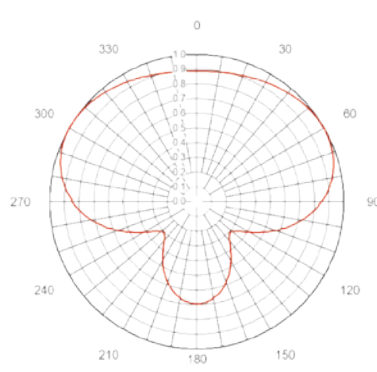
C170 1.66 (1.99 dB)
