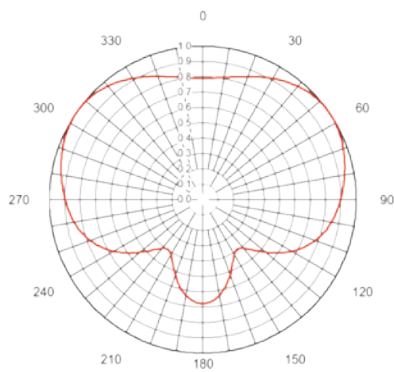
C160 1.58 (1.99 dB)
