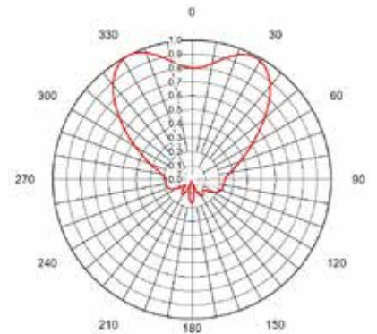
DUCKFOOT 3.74 (5.73 dB)
