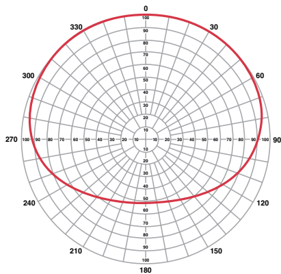
C140 DIRECTIVITY = 1.4
