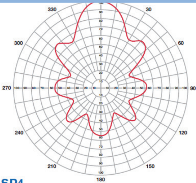
SP4 Directivity=3.0
