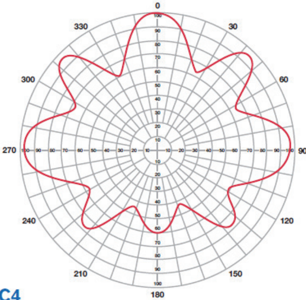
C4 Directivity=1.7
