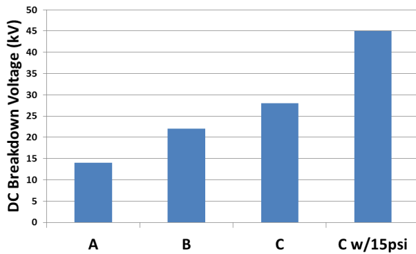
Figure 8: DC Hi-Pot testing results of tap point designs.
