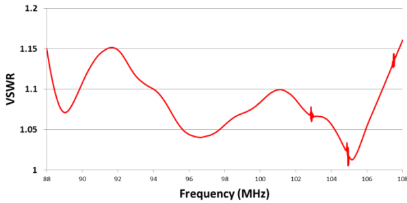
Figure 4: Measurement of a recently developed high power circularly polarized FM antenna validating the bandwidth / volume relationship developed in this paper.
