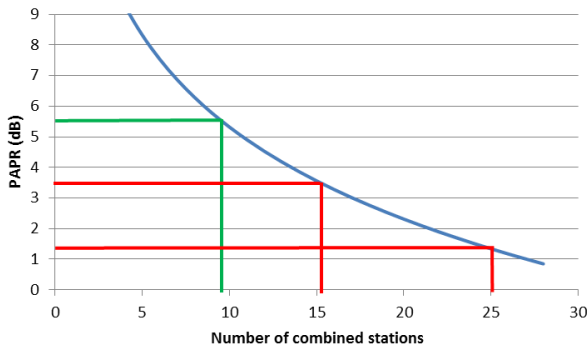
Figure 2: Number of combined stations that must be taken into account in the voltage and power handling calculations vs. PAPR of each station before a PAPR reduction factor can be applied.
