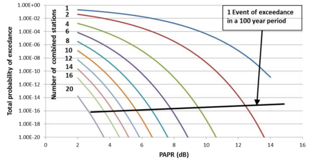
Figure 1: Recommended PAPR's to be used for total voltage handling calculations versus number of stations for a 1 time in 100 year probability of voltage breakdown. [1]
