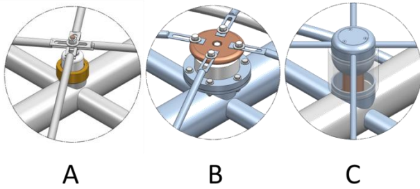
Figure 7: Tap point feed designs used on side mounted FM quadrupole ring style antennas. (A) Simple small diameter threaded inner. (B) Larger mushroom shaped tap point with rounded edges. (C) Spherical tap point with full radiuses and external pressure seal.
