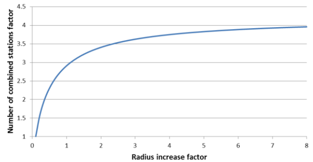
Figure 6: Relationship between increasing the radius of sharp edges and the maximum number of combined stations for a given voltage safety factor, and IBOC levels.
