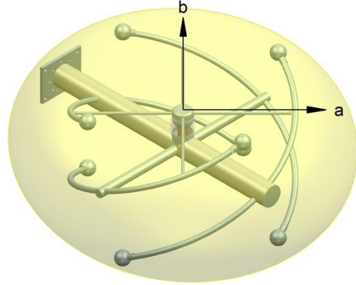
Figure 3: Full band circularly polarized side-mount quadrupole ring style antenna element fitting within an oblong bounded region.
