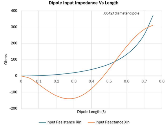
Figure 4: Input impedance vs. length of a .0042λ diameter dipole
