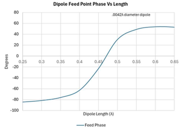
Figure 5: Feed point phase of Z_{in} vs. length of a .0042λ diameter dipole
