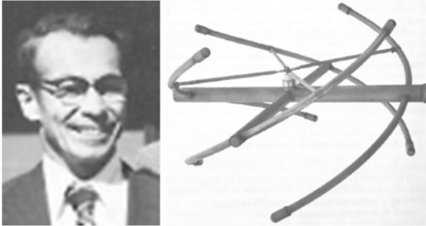
Figure 4: Don Hymas – RCA's BFM – High power broadband circularly polarized FM element.
