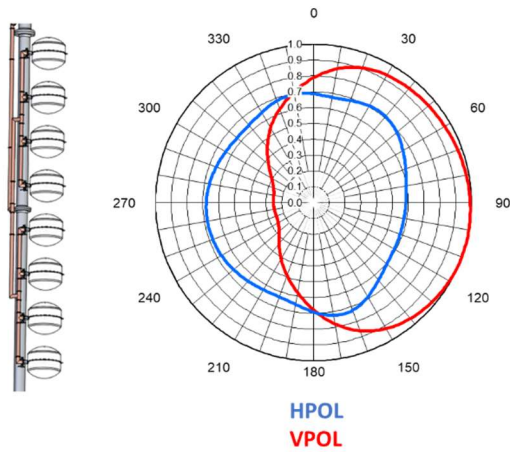
Figure 8: Horizontal and vertical polarization azimuth pattern of a FM ring style antenna when mounted to a support pole.
