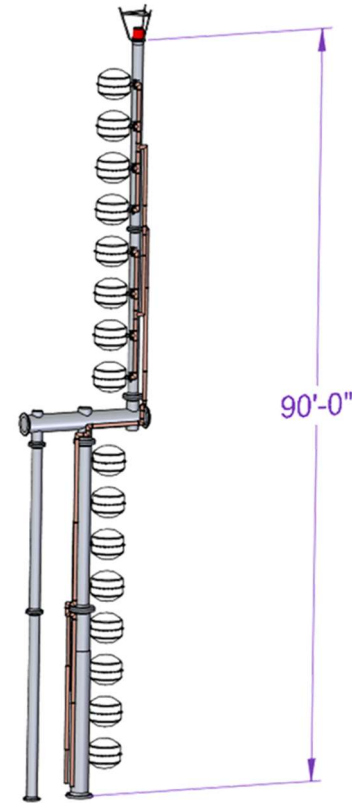
Figure 10: Full model of a 16-bay half wave spaced top mounted omni directional ring style antenna.
