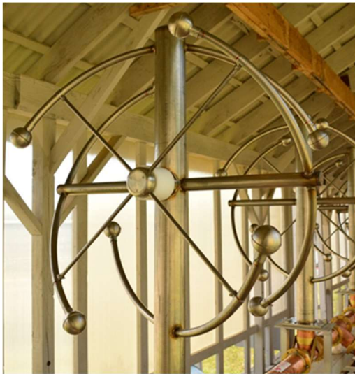
Figure 5: DCRU High power broadband ring style FM broadcast antenna bay.
