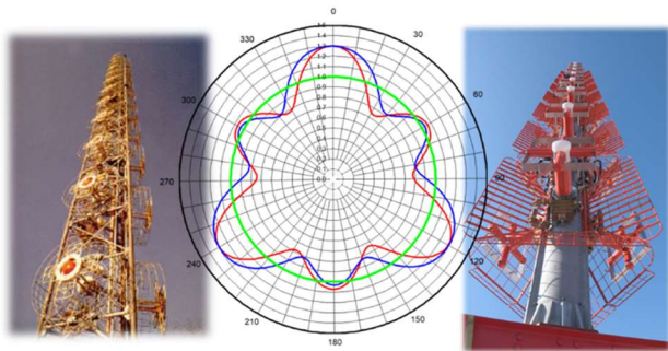
Figure 1: Top mounted high power broadband panel master FM broadcast antennas and their typical azimuth pattern performance. Blue-horizontal polarization, red-vertical polarization and green – rms.
